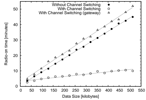
Figure 11. Average active time, with and without channel switching, for the gateway and the members of a 25-node random topology as a function of download size.
