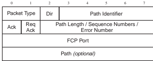
Figure 3. The FCP header.
