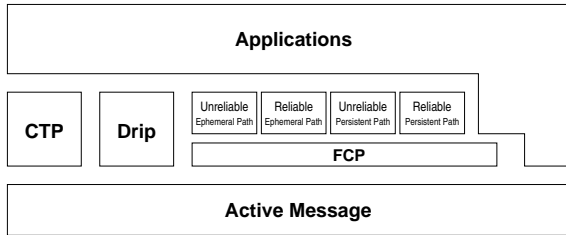
Figure 2. The Flexible Control Protocol (FCP) and its relations to other protocols in the emerging TinyOS 2 network protocol architecture.
