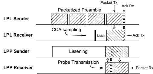
Figure 4. A simplified representation of LPL for packet-based radios and LPP. Preamble and packet durations are not drawn to scale.
